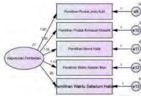
Figure 2. CFA of Endogen Variable
